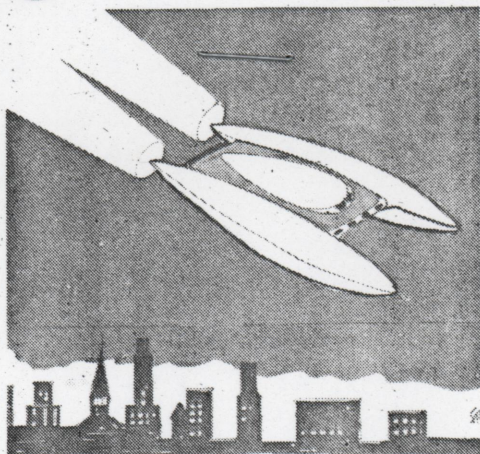
A STARSHIP'S SLOWDOWN leaves unmistakable tracks in the sky that can be detected and followed.
